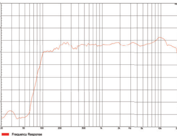
Artist T43 Frequency Response Curve
